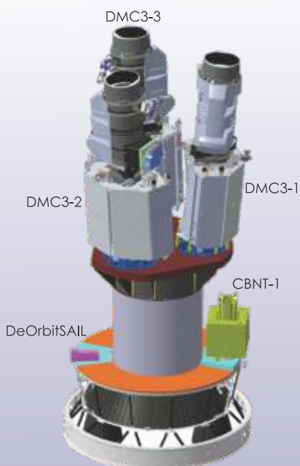
Location of payloads on the mounting adopters of PSLV-C28
