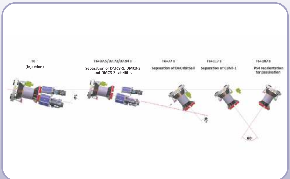
Separation details of PSLV-C28 payloads
