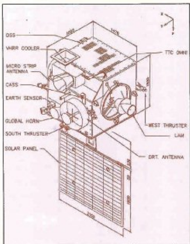
Identification of systems on Metsat
