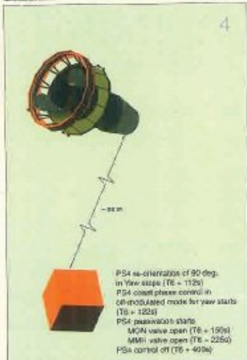
PS4 orientation sequence for spacecraft separation and passivation
